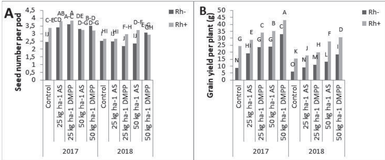
Figure 4. The interaction between rhizobia and different nitrogen fertilization on seed number per pod (A) and grain yield per plant (B) of bean. Letters on each bar represent significance level at P < 0.05 .
